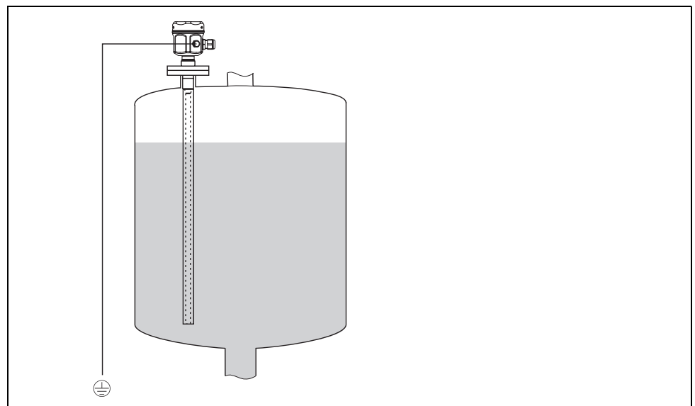
Probe with ground tube and grounding
