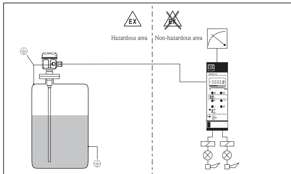
Level measurement
