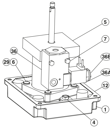
Typical Cylinder Assembly Mounting
